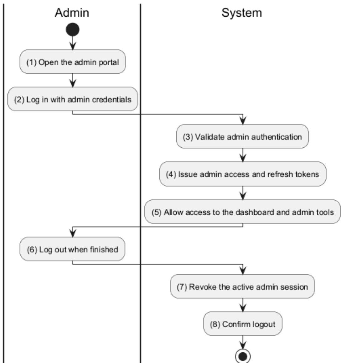
Figure 3.30: Activity Diagram for UC-29
