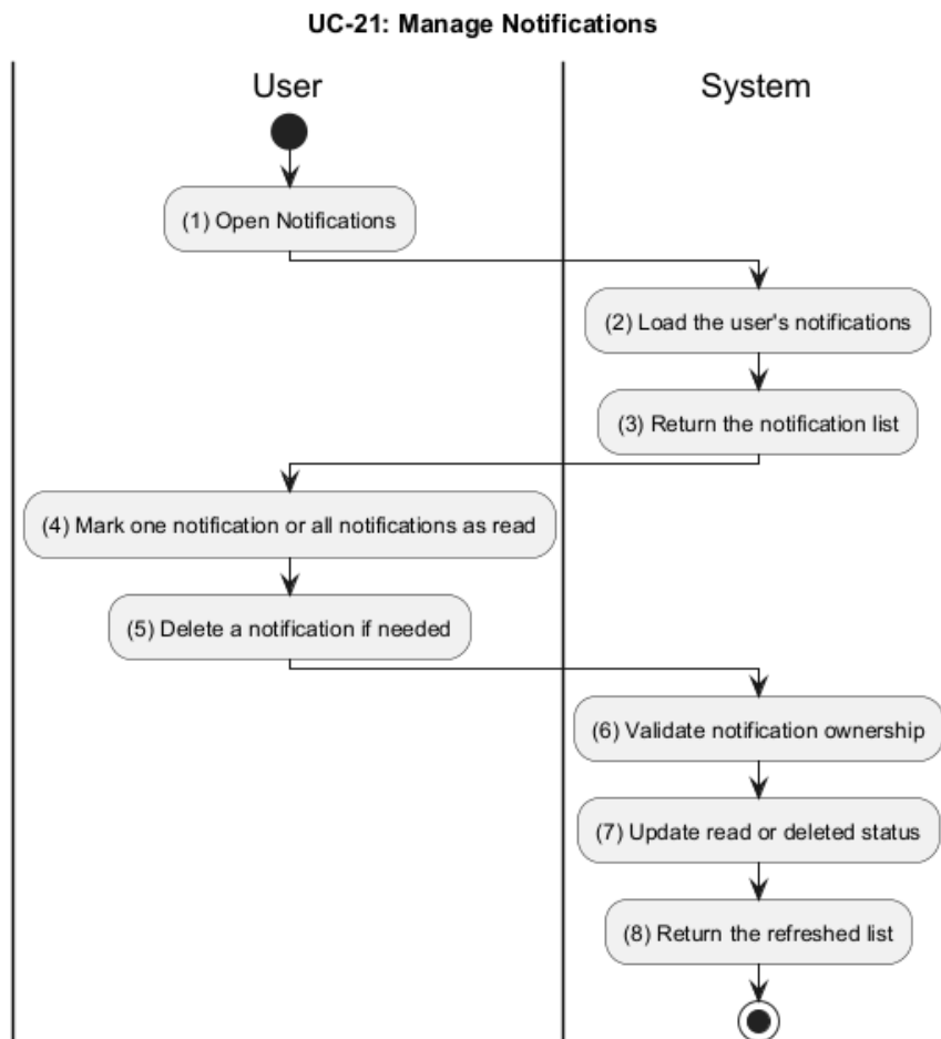
Figure 3.22: Activity Diagram for UC-21
