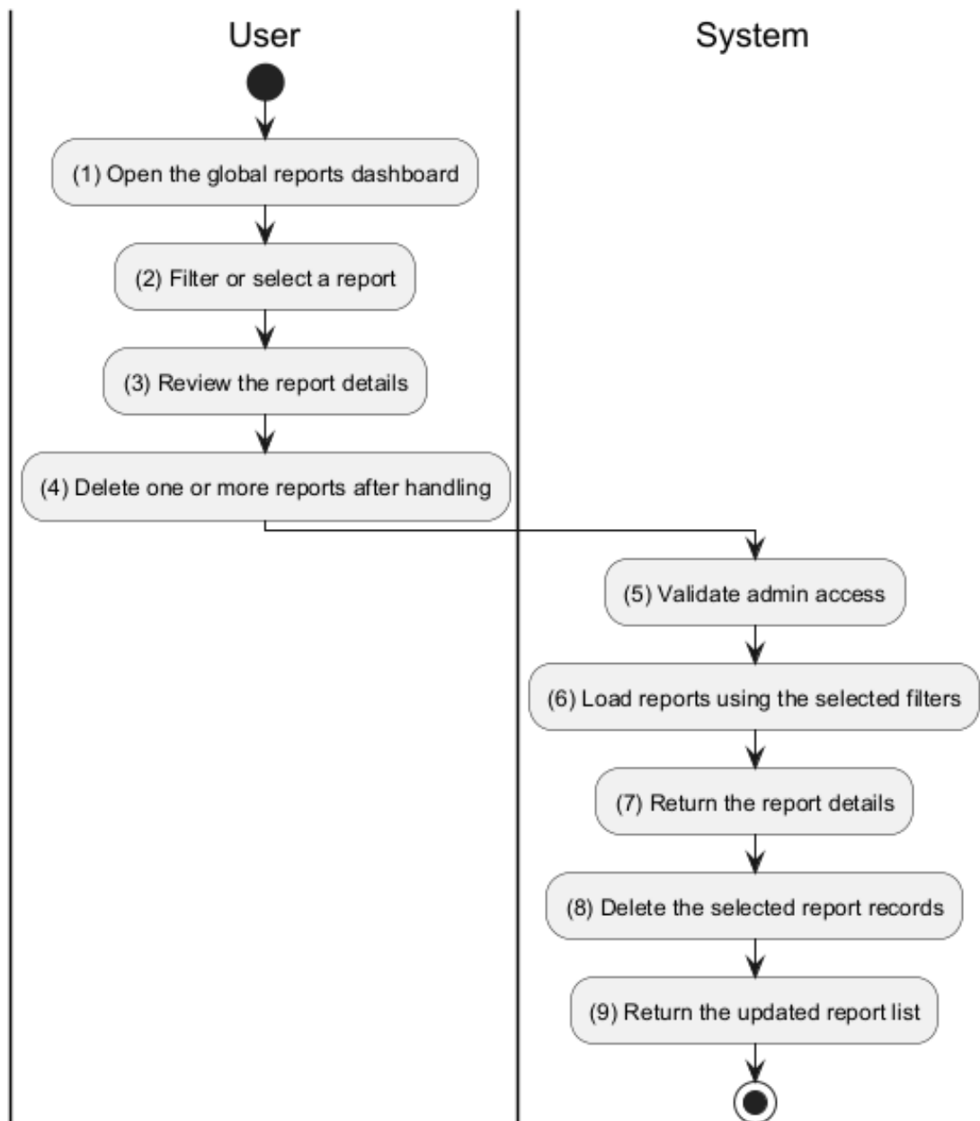
Figure 3.29: Activity Diagram for UC-28
